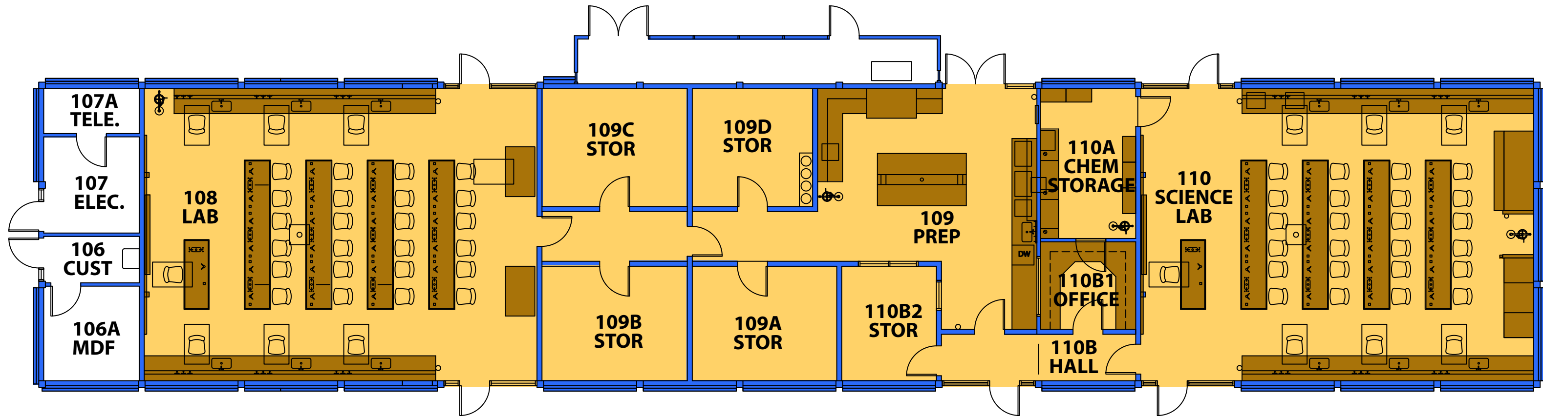
#01 CLASSROOM NORTH WING FLOOR PLAN
